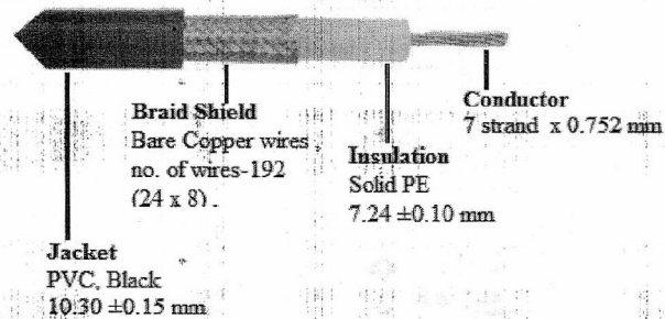
RG 213 Coaxial Cable Construction
